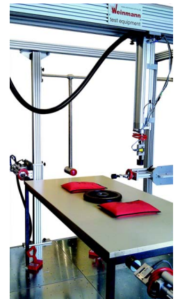
Pendulum impact hammer with angle scala
