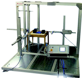
Placing profile for free setting up of the operating stamp in the test field
